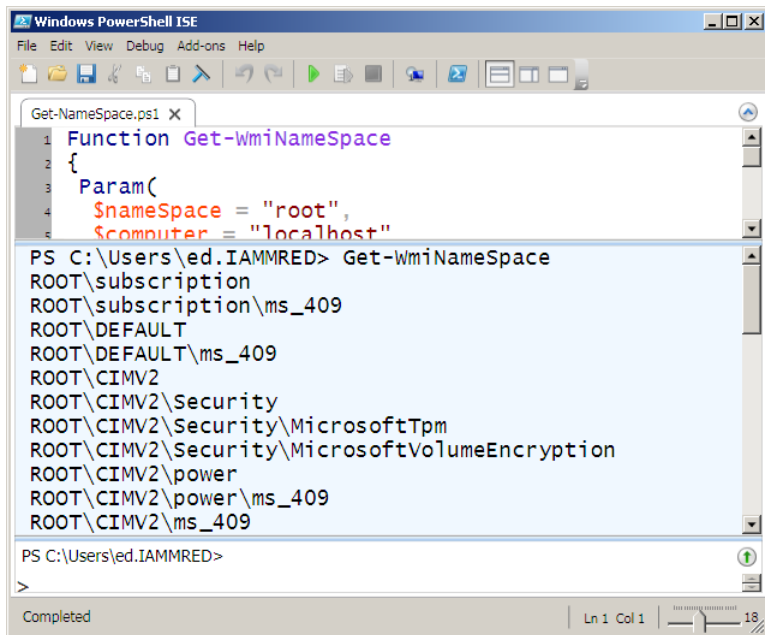
FIGURE 10-3 WMI namespaces revealed by the Get-WmiNameSpace function.
