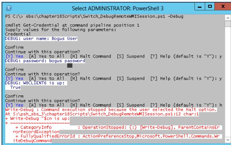
FIGURE 18-4 Using the -debug switched parameter to step through potential problems in a script.
